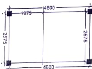
LAYOUT PLAN
