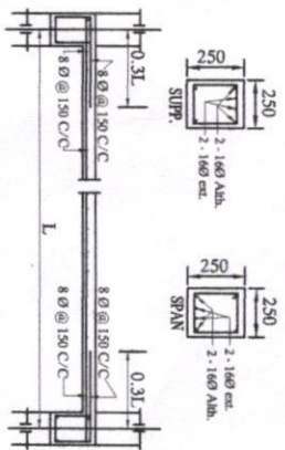
Details Of R.C.C Roof Slab & Beam
