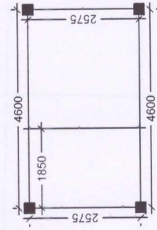
LAYOUT PLAN
