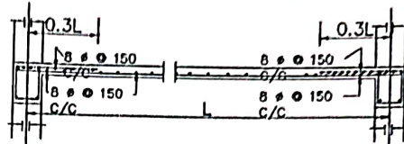
Details Of R.C.C Roof Slab & Beam
