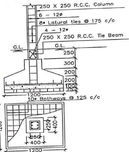
DETAILS OF R. C. C COLUMN (SCALE - 1 : 25)
