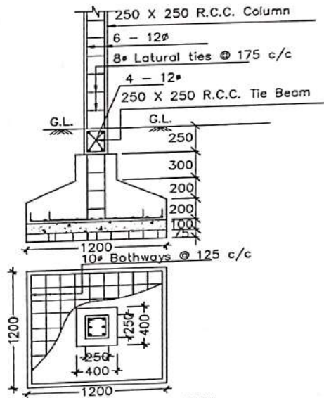
DETAILS OF R. C. C COLUMN (SCALE - 1 : 25)
