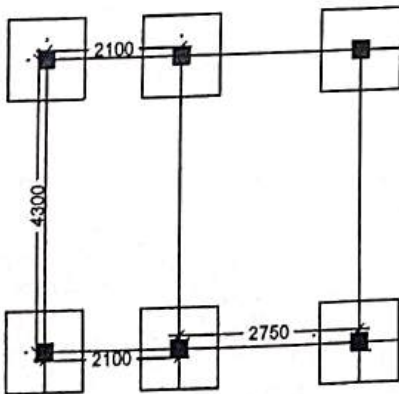
LAYOUT PLAN
