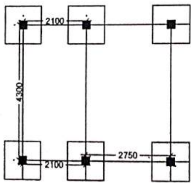
LAYOUT PLAN
