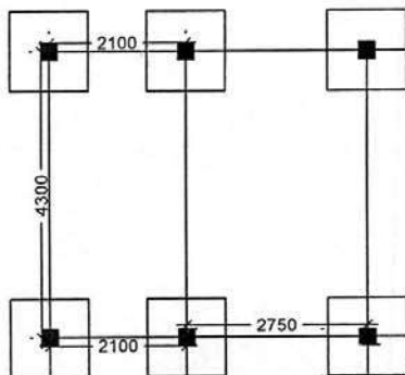
LAYOUT PLAN
