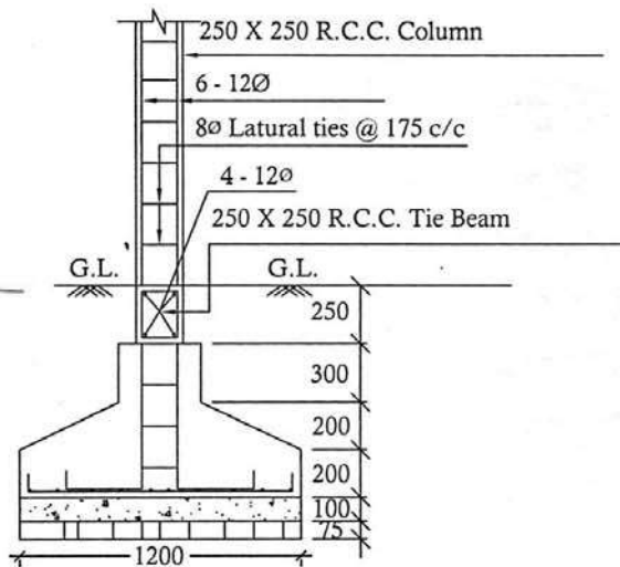
10Ø Bothways @ 125 c/c
