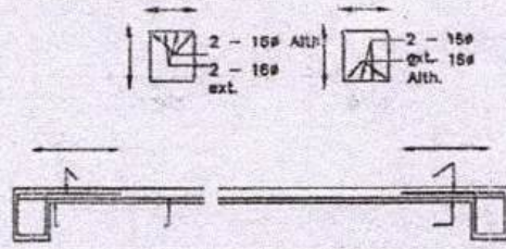
Details Of R.C.C Roof Slab & Beam
