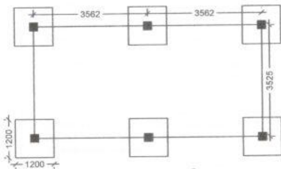
LAYOUT PLAN
