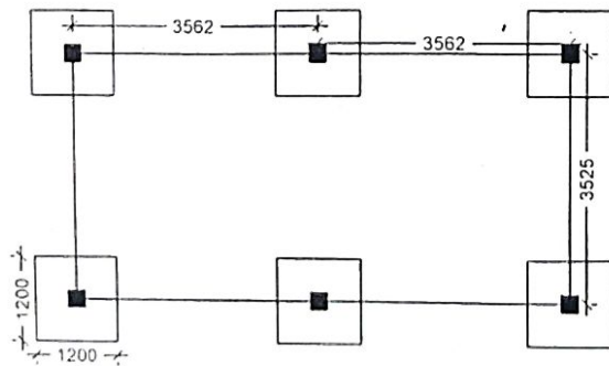
LAYOUT PLAN
