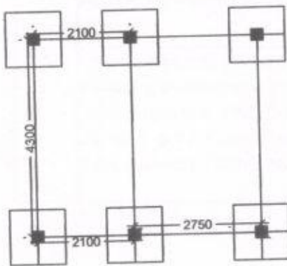
LAYOUT PLAN
