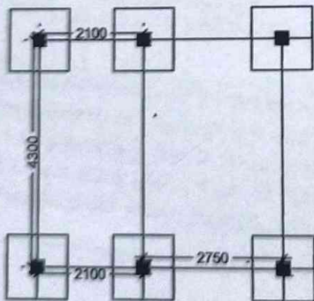
LAYOUT PLAN
