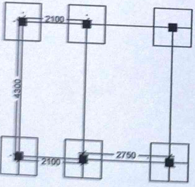
LAYOUT PLAN
