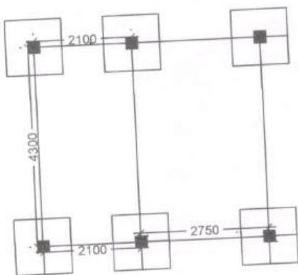
LAYOUT PLAN
