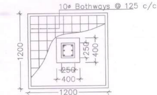
DETAILS OF R. C. C COLUMN (SCALE - 1 : 25)
