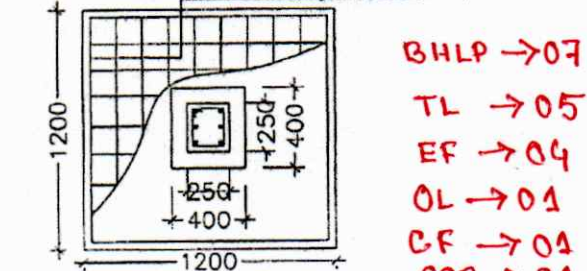
DETAILS OF R. C. C COLUMN (SCALE - 1 : 25)
