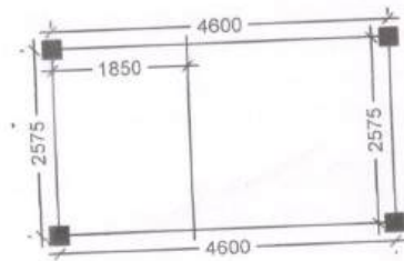
LAYOUT PLAN
