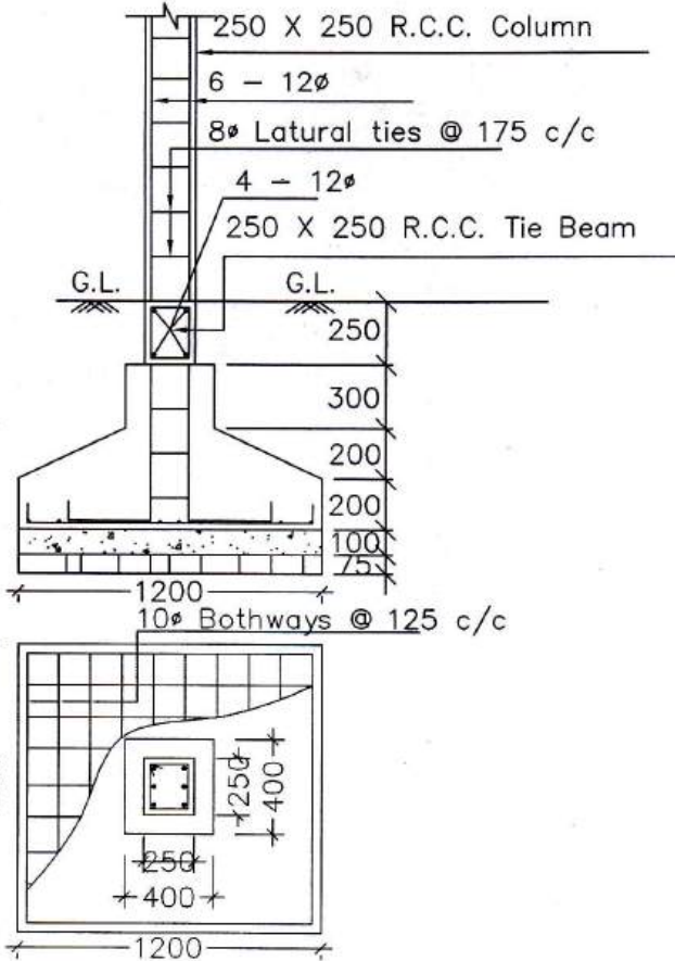
DETAILS OF R. C. C COLUMN
