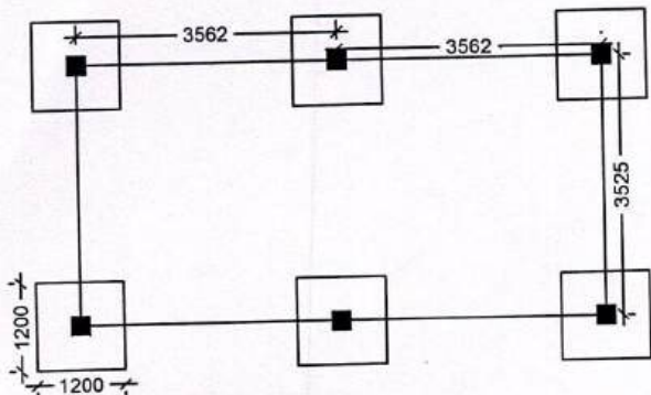
LAYOUT PLAN
