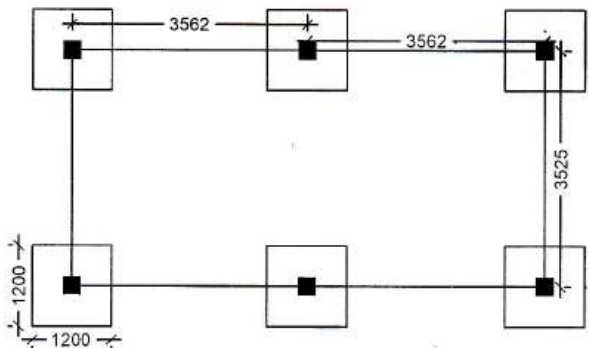
LAYOUT PLAN
