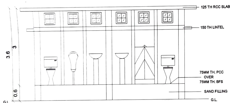
CROSS SECTIONAL VIEW AT X-Y
