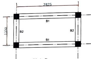
Slab Beam Details
