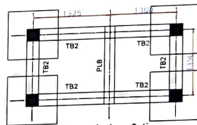
Foundation & tie Beam Details
