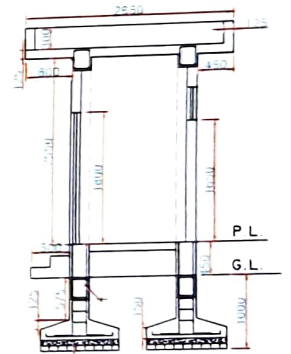
DETAILS OF WALL SECTION A-A
