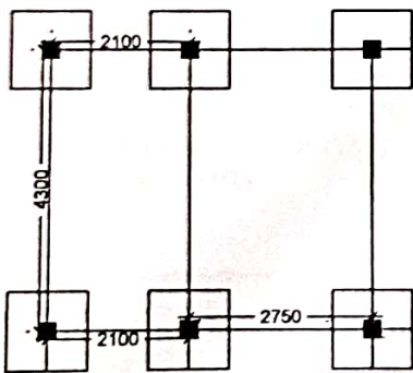
LAYOUT PLAN
