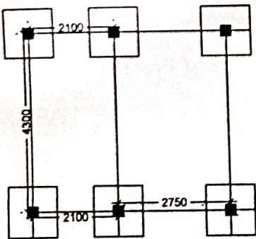
LAYOUT PLAN
