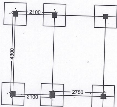
LAYOUT PLAN
