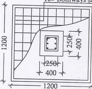
DETAILS OF R. C. C COLUMN (SCALE - 1 : 25)
