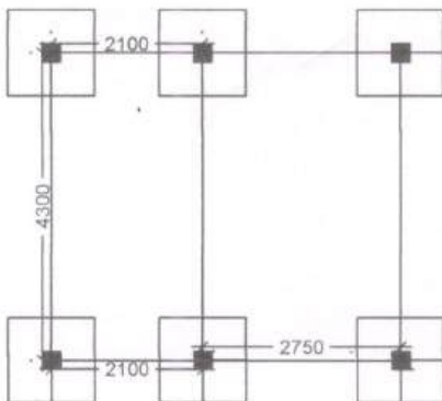
LAYOUT PLAN
