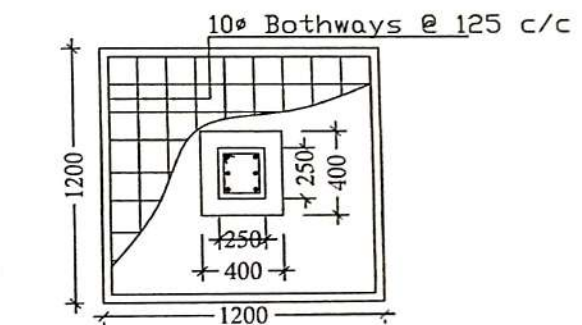
DETAILS OF R. C. C COLUMN
