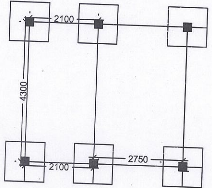
LAYOUT PLAN
