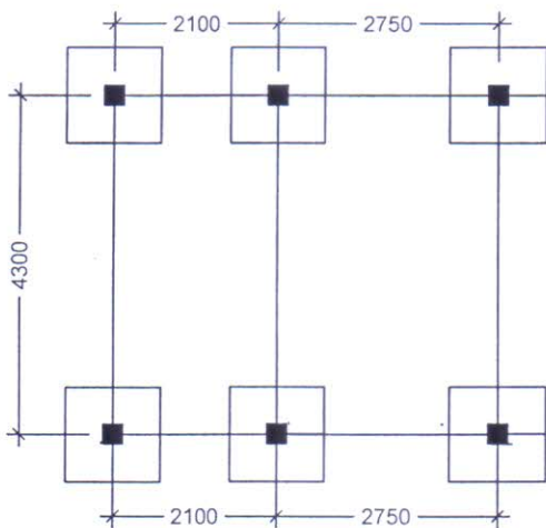
LAYOUT PLAN
