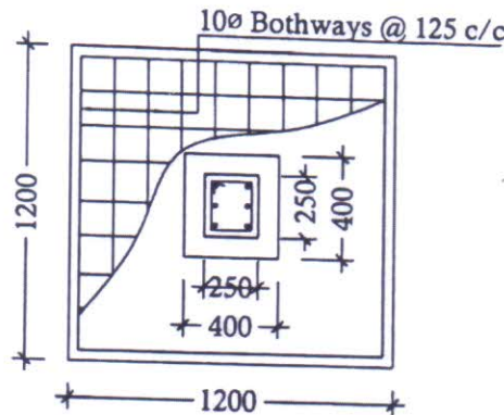
DETAILS OF R. C. C COLUMN (SCALE - 1 : 25)
