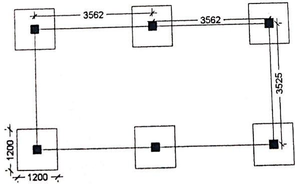
LAYOUT PLAN
