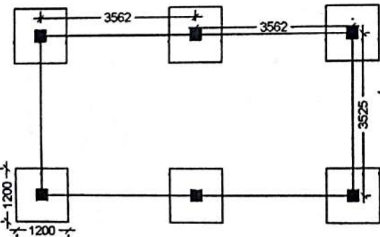
LAYOUT PLAN
