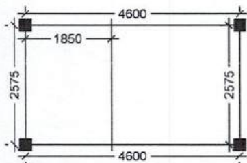
LAYOUT PLAN
