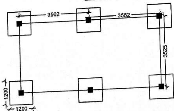
LAYOUT PLAN
