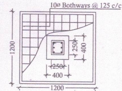
DETAILS OF R. C. C COLUMN
