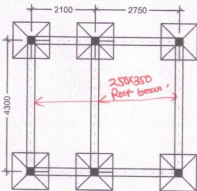
LAYOUT PLAN
