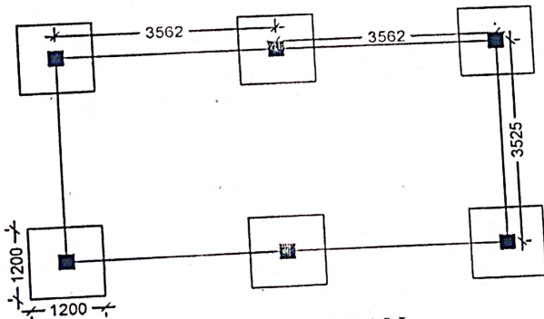
LAYOUT PLAN
