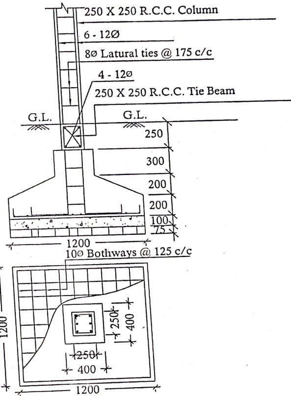
DETAILS OF R. C. C COLUMN
