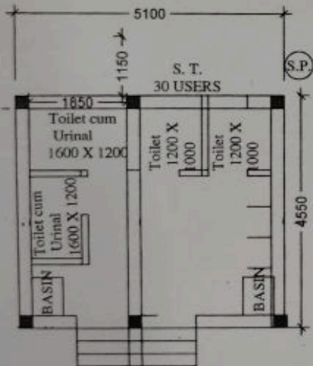
PLAN
