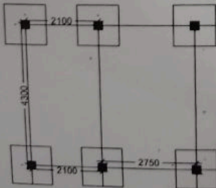
LAYOUT PLAN
