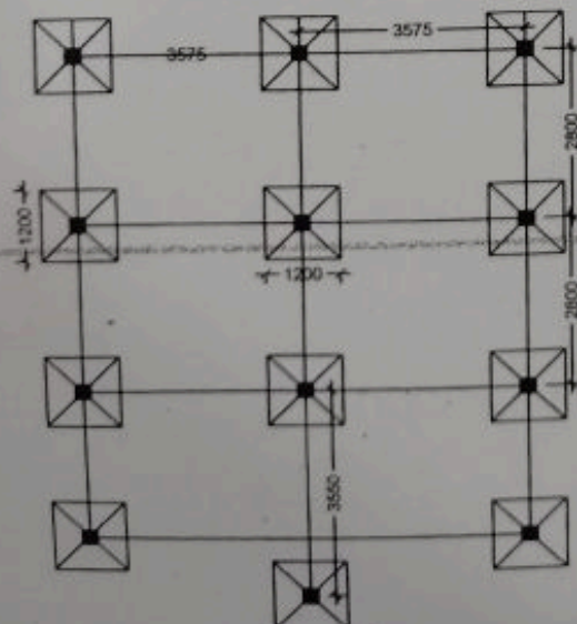
LAYOUT PLAN
