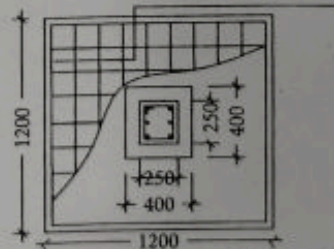
DETAILS OF R.C.C COLUMN (SCALE - 1 : 25)
