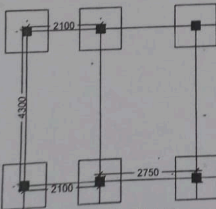
LAYOUT PLAN
