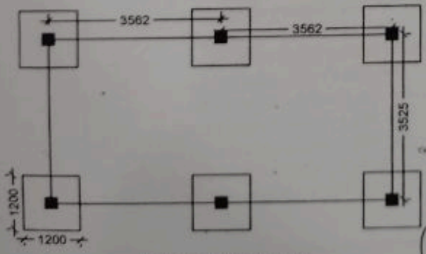
LAYOUT PLAN
