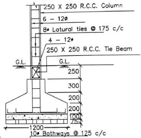
DETAILS OF R. C. C COLUMN (SCALE - 1 : 25)
