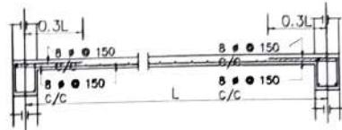
Details Of R.C.C Roof Slab & Beam (SCALE - 1 : 25)
