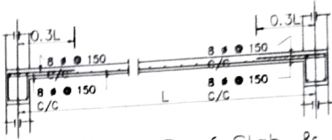
Details Of R.C.C Roof Slab & Beam (SCALE - 1 : 25)
