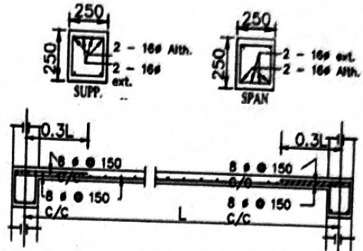
Details Of R.C.C Roof Slab & Beam (SCALE - 1 : 25)
