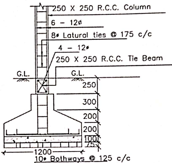
DETAILS OF R. C. C COLUMN (SCALE - 1 : 25)
