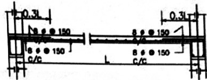
Details Of R.C.C Roof Slab & Beam
