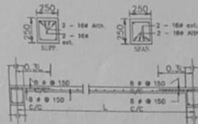
Details Of R.C.C Roof Slab & Beam (SCALE - 1 : 25)
