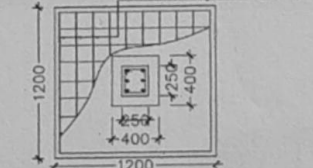
DETAILS OF R. C. C COLUMN (SCALE - 1 : 25)
