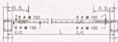
Details Of R.C.C Roof Slab & Beam
