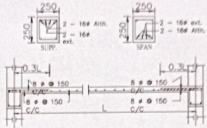
Details Of R.C.C Roof Slab & Beam
